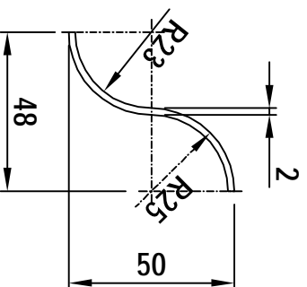
Lamelle "KS - 50"
