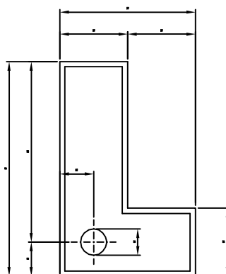
Rinne in L-Form
